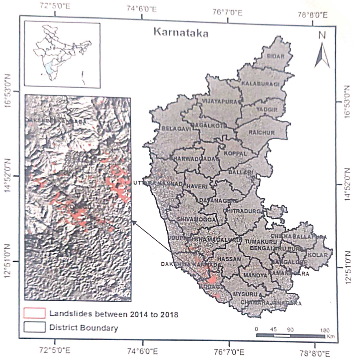
Figure 39. Landslides mapped using high-resolution satellite data in Karnataka, which occurred between 2014 to 2018.
