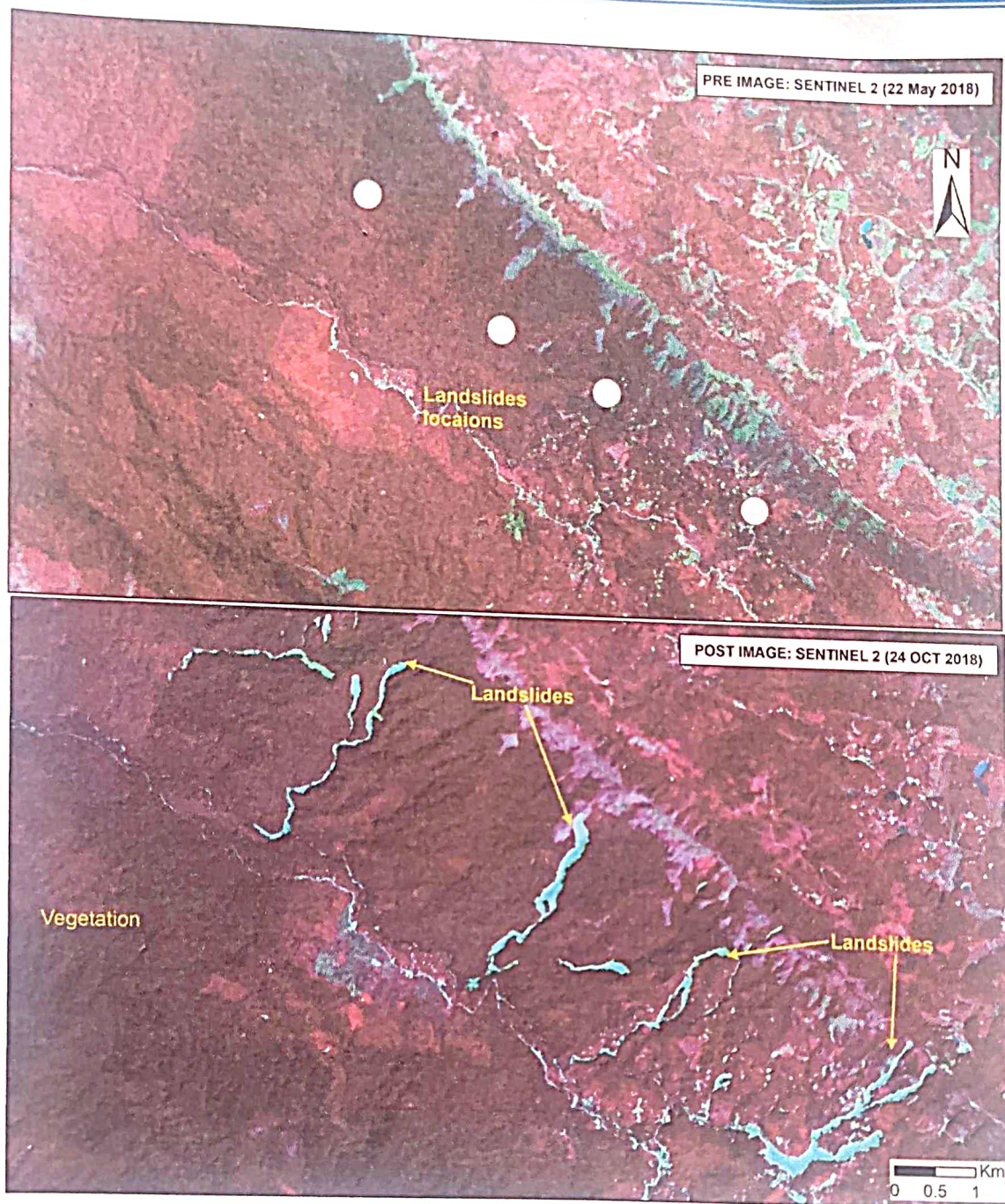
Figure 40. Landslide from Kodagu and Dakshina Kannada districts, Karnataka. Landslides were triggered in the Kodagu and Dakshina Kannada districts of Karnataka due to heavy rain in the 3rd week of August, 2018. Majority of the landslides were shallow translational failures.
